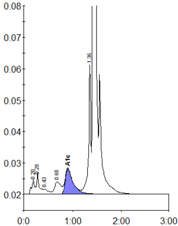
Peak table - ID: 10431877
